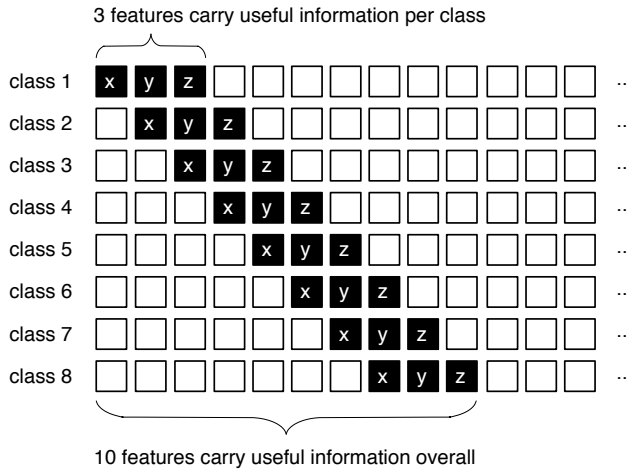
Fig. 4 Illustration of the coordinate feature placement for the cube dataset. The white boxes resemble random features which carry no useful information for the classification task. The black x, y, and z boxes are the informative features that describe a coordinate in three-dimensional space. The coordinate features are shifted by one position for each class. Conventional FS methods can only select features independent of the class and thus their best possible outcome is to choose the 10 features that carry useful information.
