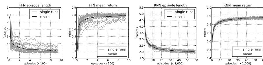
Fig. 6 Results of MNIST with FFN (left two plots) and RNN (right two plots). For each classifier, mean episode length and mean return over training episodes are shown.
