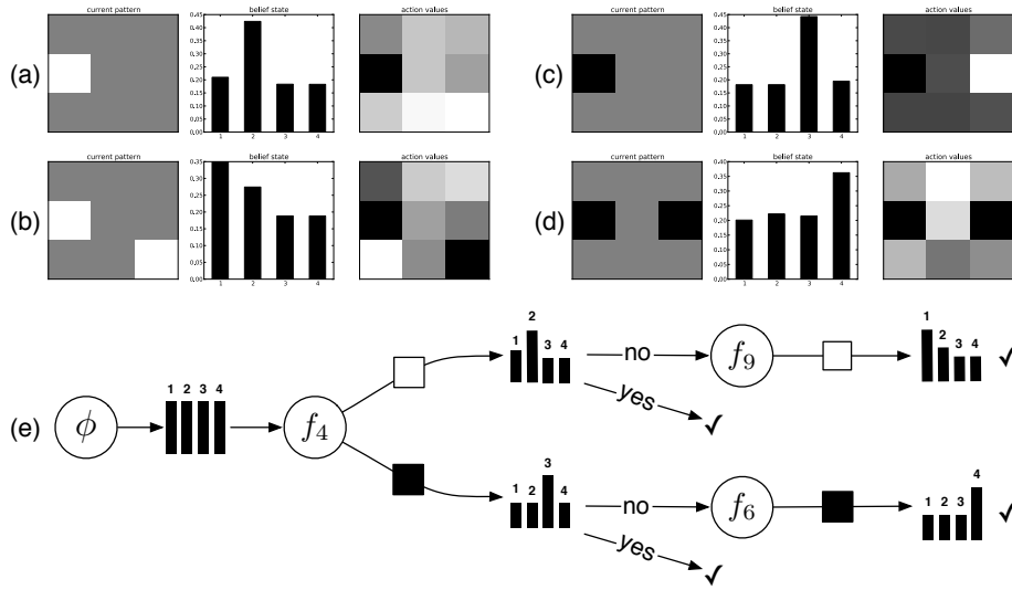
Fig. 2 Decision process of the SOFS agent after training. (a)–(d) each show the already uncovered features in the explicit memory (left), the belief state histogram (middle) and the action value table for selecting the next feature (right, white indicates high values). (e) shows the decision process graphically. Initially the agent always sees the missing value and chooses to look at feature 4 first. If the feature is white, the classifier favours class 2, and SOFS proposes to select feature 9, should it be wrong (a). After looking at feature 9, the classifier then favours class 1 (b). If feature 4 was black, however, the classifier favours class 3 and SOFS suggests to select a different feature next, namely feature 6 (c). After looking at it, the classifier now favours class 4 (d).
