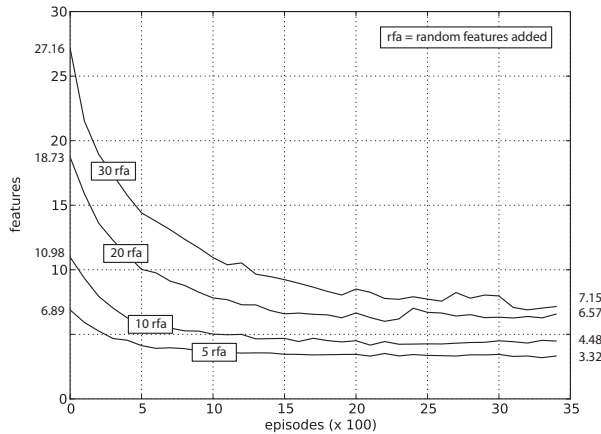
Fig. 5 Results of the SOFS training process on the cube dataset. The four plots show instances of the dataset with a different number of random features added (rfa) to the 3 informative features. In all cases, SOFS learns to ignore most of the random features and mostly focuses on the informative ones. However, the more random features were added, the more difficult it is to find the 3 coordinates. Initial number of features before training and final number of features are displayed at the axis sides left and right respectively.
