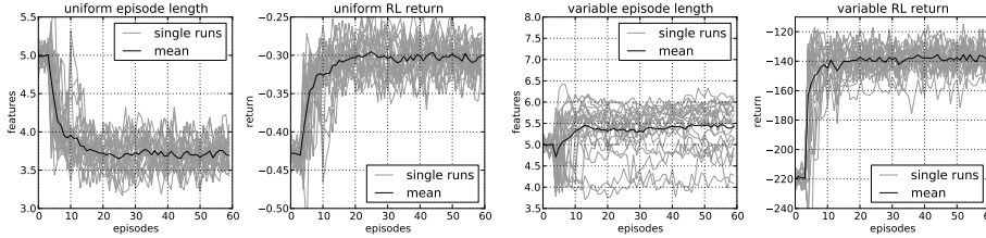
Fig. 7 Results of the PIMA diabetes dataset with Naive Bayes classification. Left two figures: episode lengths and mean returns for uniform feature costs. Right two figures: episode lengths and mean returns for feature costs according to Table 1.
